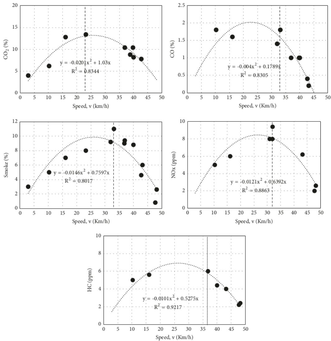
FIGURE 5: Exhaust emission driving cycle pattern on good road conditions.
